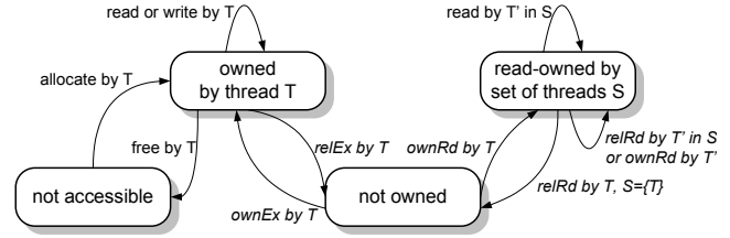
Figure 1. Core ownership states.
