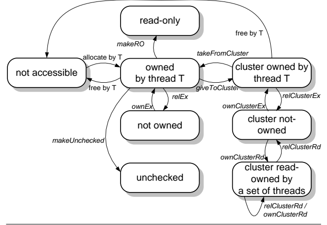
Figure 9. Memory ownership states.
